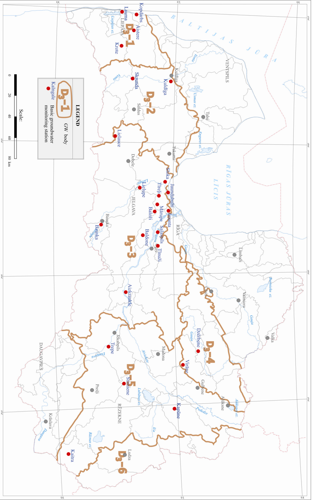
Distribution of groundwater monitoring stations within GW bodies of Famennian - Permian and Plavinas - Amula multi-aquifer systems
