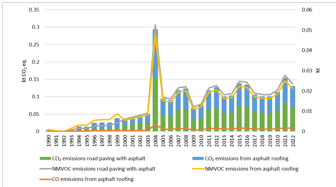
Figure 4.14 Emissions from asphalt roofing and road paving in 1990–2022 (NMVOC and CO emissions on secondary axis) (kt CO 2 eq.; kt)
