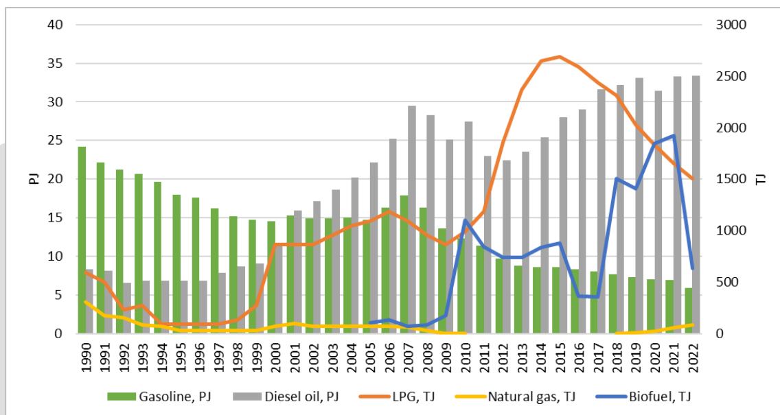
Figure 3.28 Development of Fuel consumption in road transport (PJ;TJ) 26
