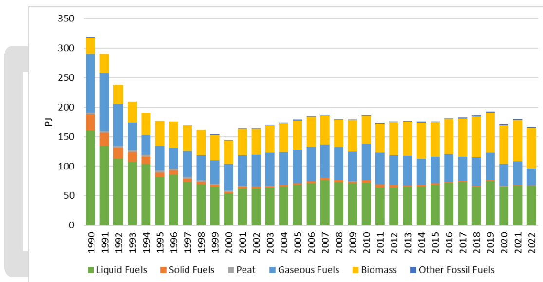
Figure 2.5 Fuel consumption in Energy sector 1990-2022 (PJ)
