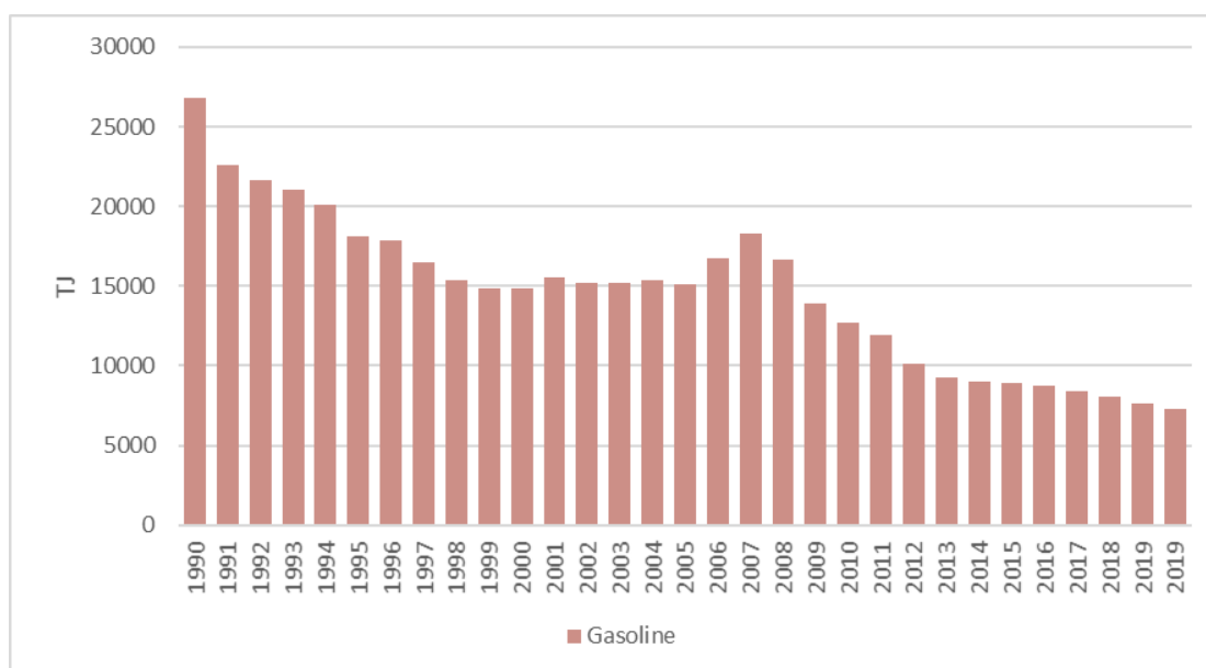
Figure 3.23 Gasoline consumption in Latvia in 1990-2020, TJ
