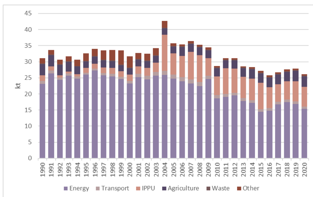
Figure 2.7 Total PM 10 emissions, kt
