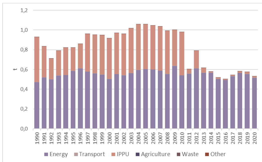
Figure 2.11 Total Cd emissions (t)
