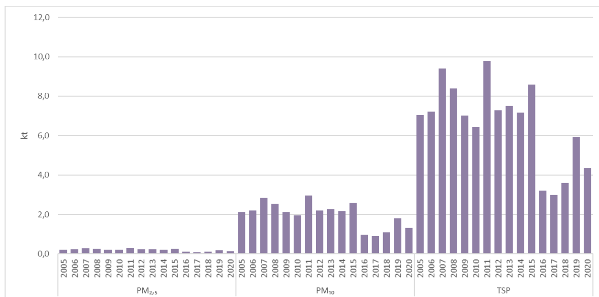
Figure 4.6 Particulate matter emissions from building and road construction in 2005-2020, kt
