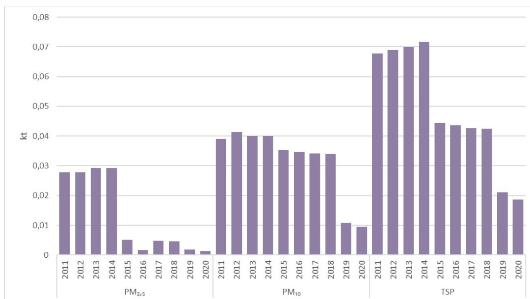
Figure 4.7 PM emissions from storage, handling and transport of mineral products 2011-2020, kt
