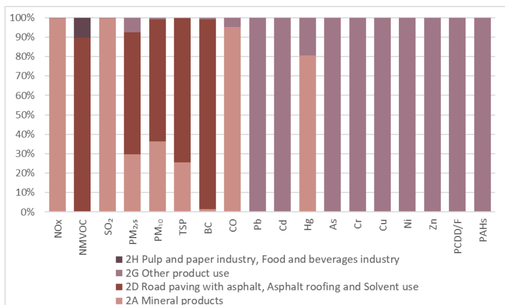
Figure 4.1 Emissions from Industrial processes and product use sector by subsectors in 2020
