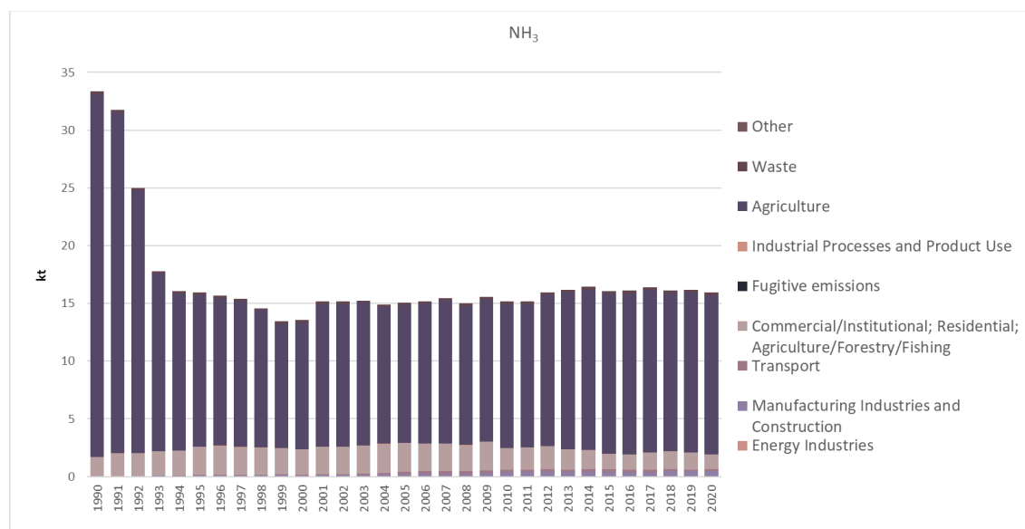
Figure 2.4 Total NH 3 emissions, kt
