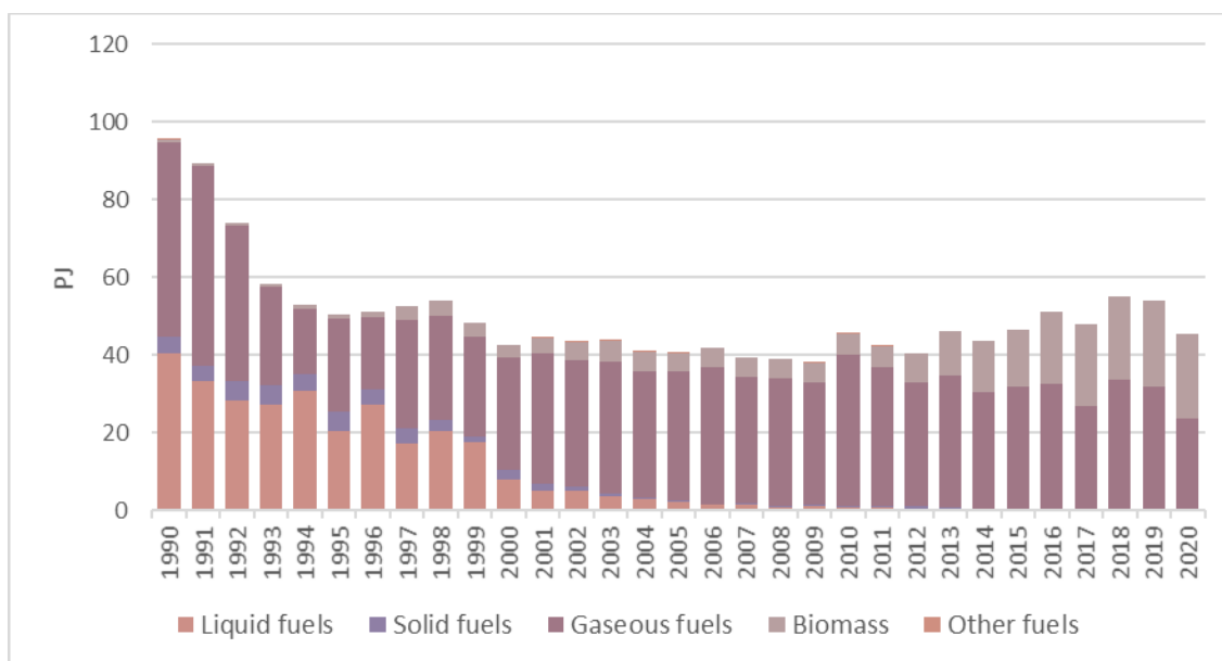
Figure 3.2 Fuel consumption in NFR 1A1 Energy Industries in 1990-2020, PJ
