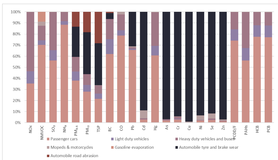
Figure 3.7 Emissions in Road transport, 2020
