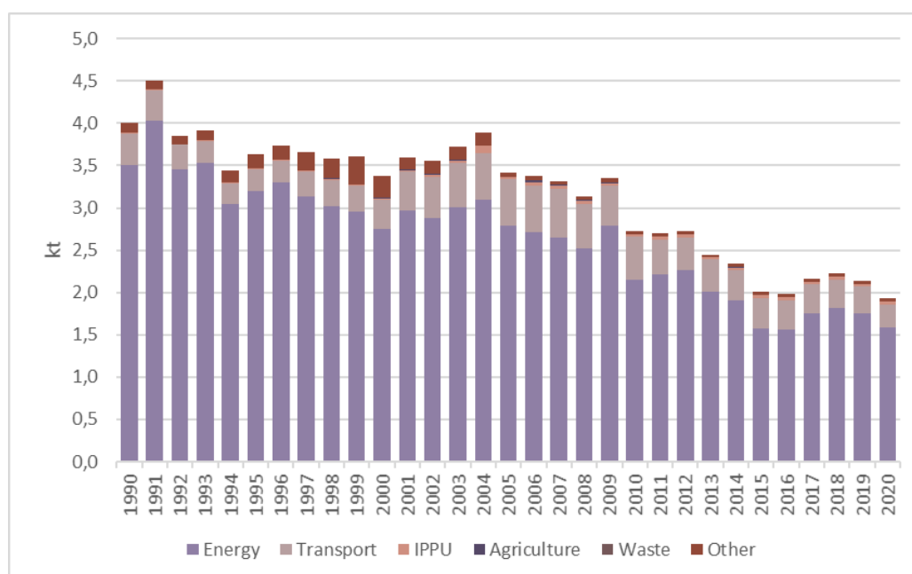
Figure 2.9 Total BC emissions, kt
