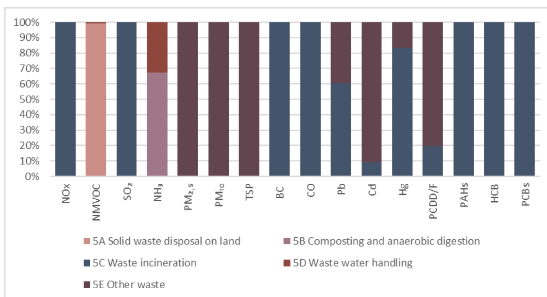
Figure 6.1 Distribution of emissions in Waste sector by subsectors in 2020, %
