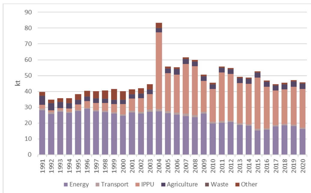
Figure 2.8 Total TSP emissions, kt
