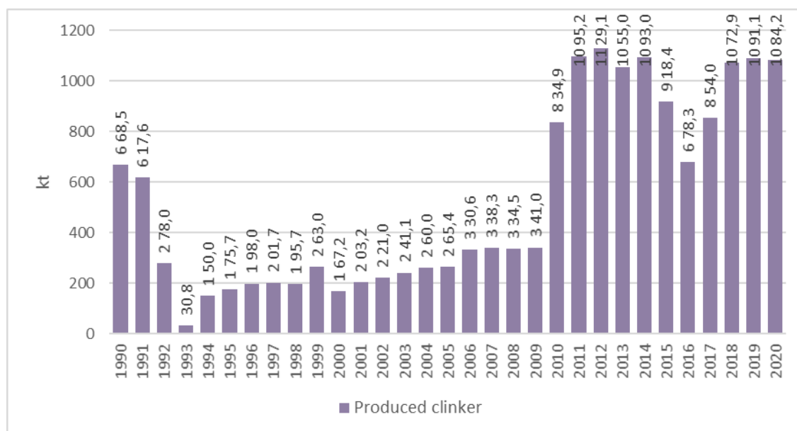
Figure 4.2 Cement production activity data in 1990-2020, kt
