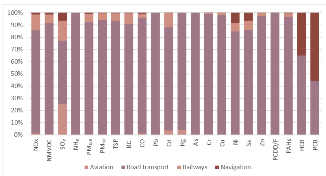
Figure 3.5 Distribution of emissions in Transport sector by subsectors in 2020, %
