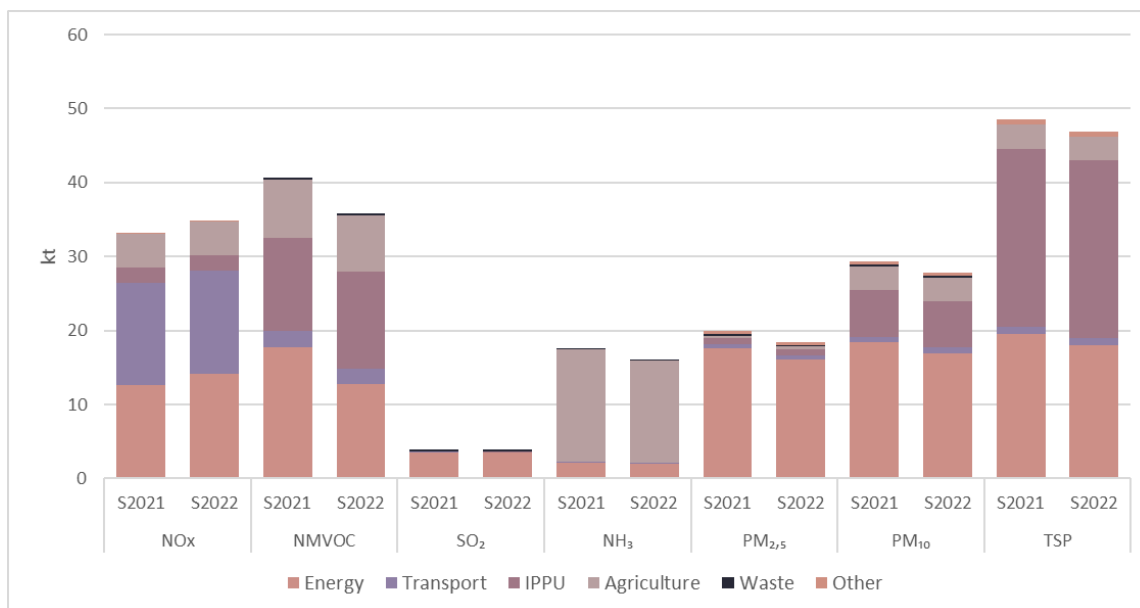
Figure 8.1 Emission comparison for 2019 between IIR Submission 2021 and IIR Submission 2022
