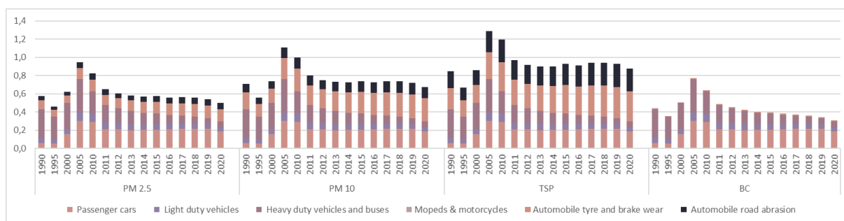
Figure 3.9 Distribution of solid particle emissions by sources in Road transport, kt
