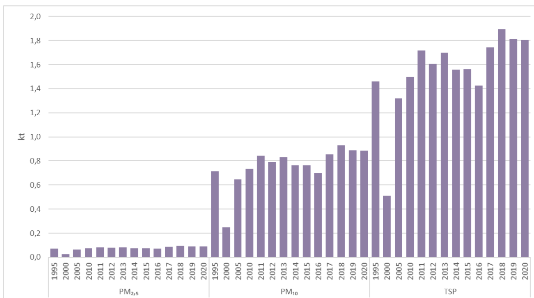
Figure 4.5 Particulate matter emissions from quarrying of minerals in 1995-2020, kt
