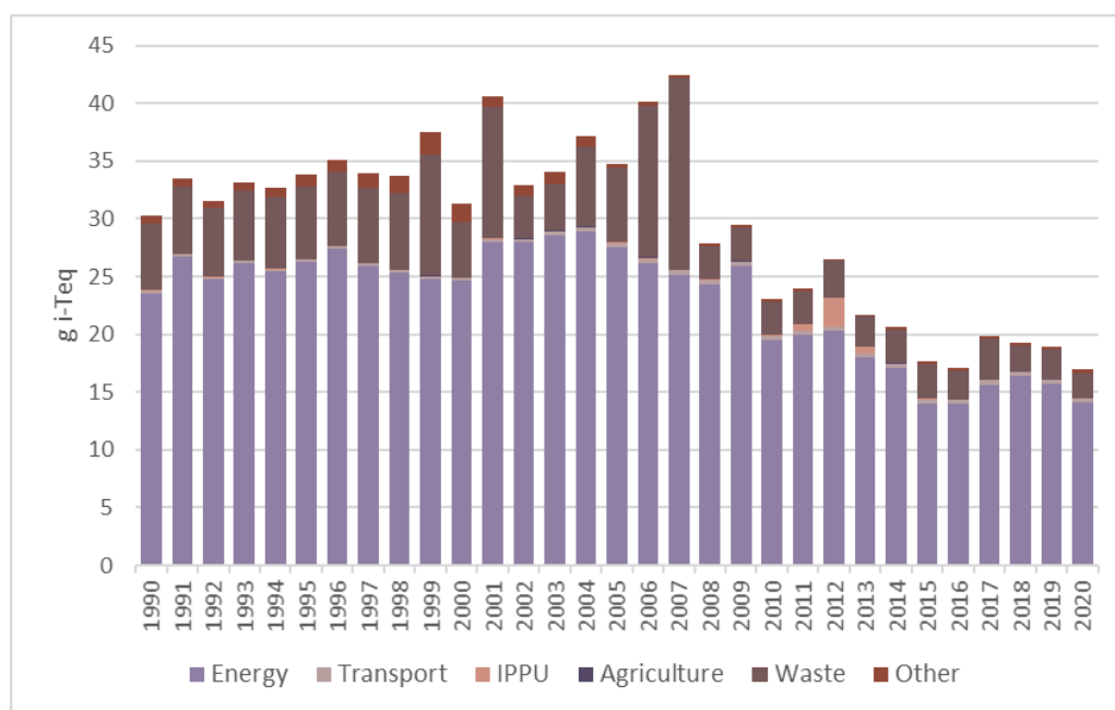
Figure 2.13 Total PCDD/F emissions (g i-Teq)
