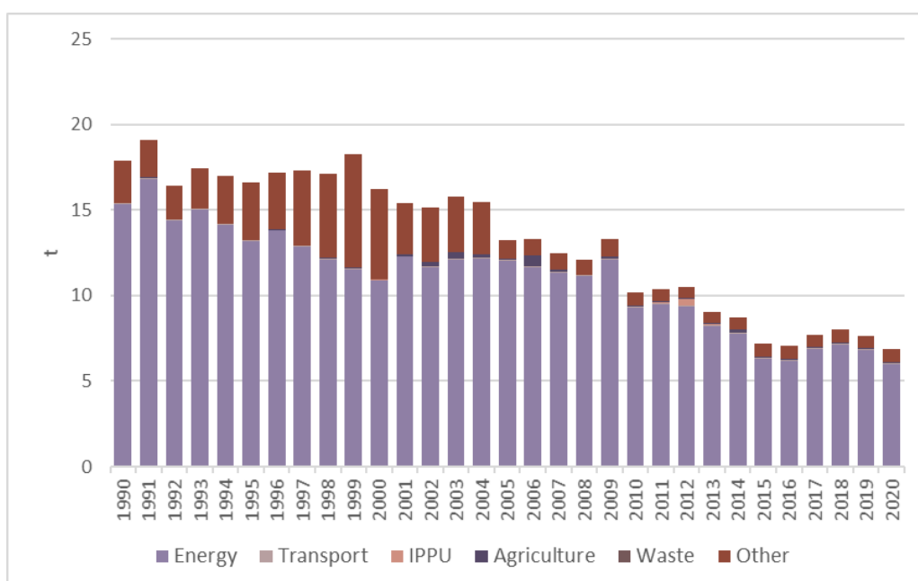
Figure 2.14 Total PAH emissions (t)
