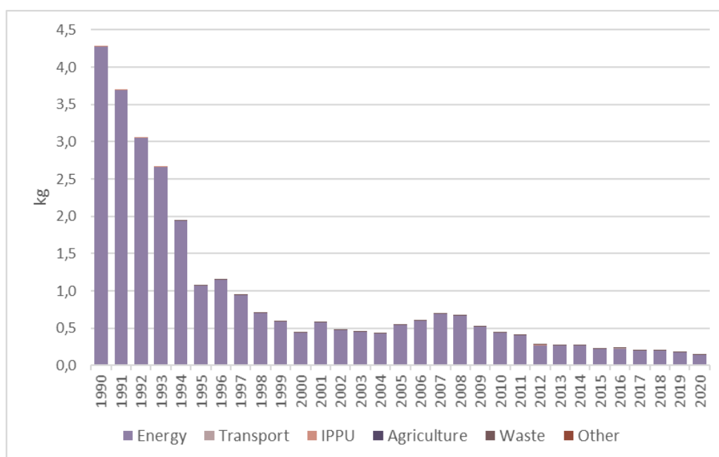
Figure 2.16 Total PCB emissions (kg)
