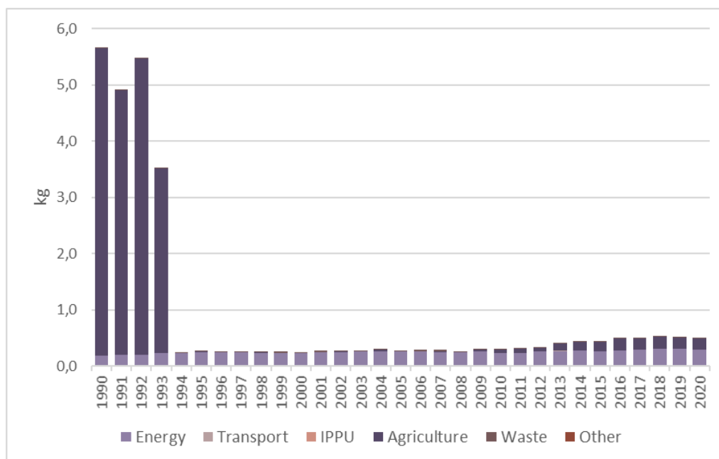
Figure 2.15 Total HCB emissions (kg)
