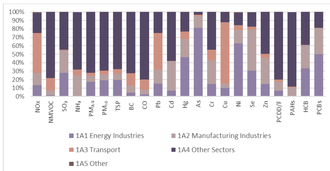
Figure 3.1 Distribution of emissions from Fuel combustion in 2020, %
