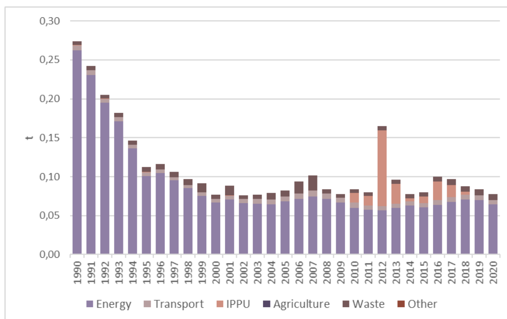
Figure 2.12 Total Hg emissions (t)
