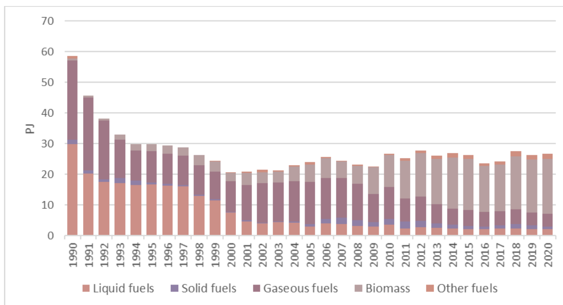
Figure 3.4 Fuel consumption in NFR 1A2 Manufacturing Industries and Construction in 1990-2020, PJ
