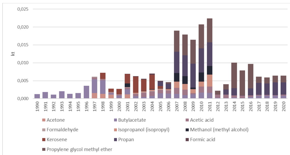
Figure 4.4 NMVOC emissions from glass fibre production in 1990-2020, kt
