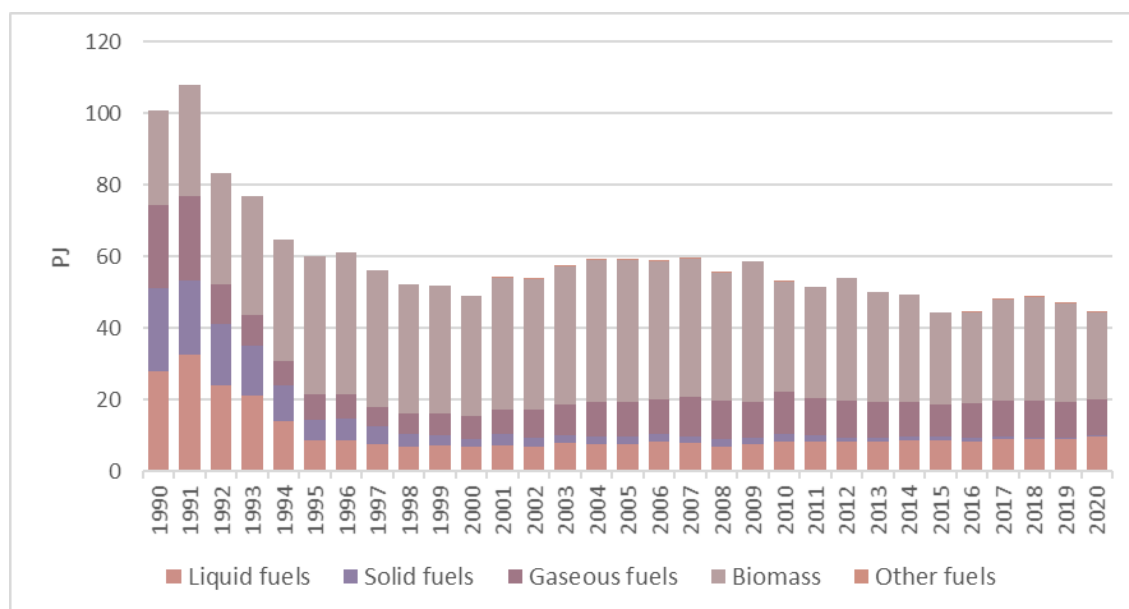
Figure 3.20 Fuel consumption in NFR 1A4 Other Sectors in 1990-2020, PJ
