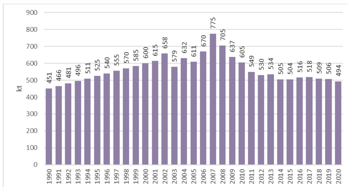
Figure 6.3 Disposed waste amount in Latvia, kt
