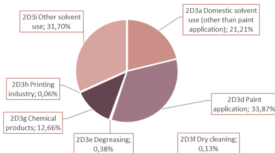
Figure 4.9 Distribution of NMVOC emissions in Solvent use sector in 2020, kt
